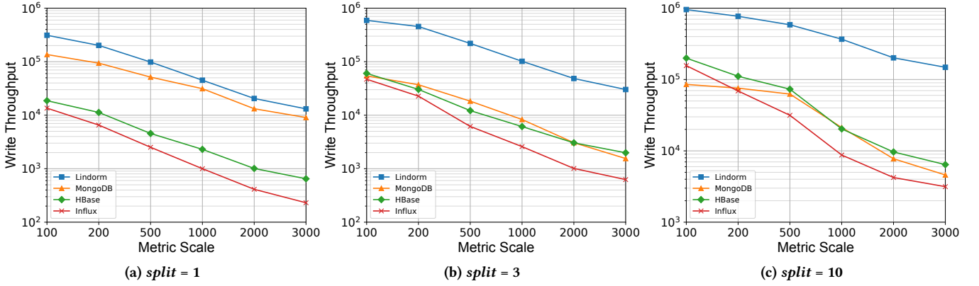
Figure 11: Write throughput at different split and metric_scale .
