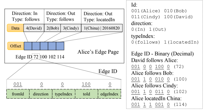
Figure 6: The storage structure within a single Edge Page and the composition of Edge ID
