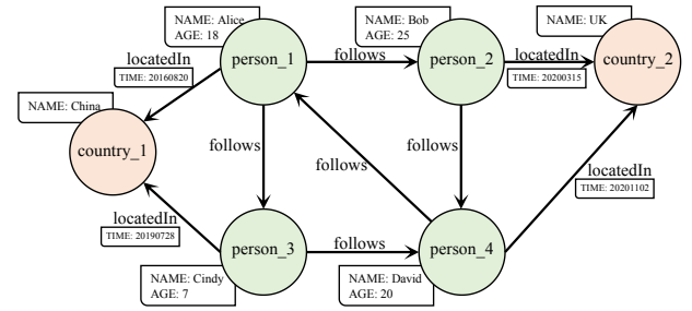
Figure 1: An example of property graph
