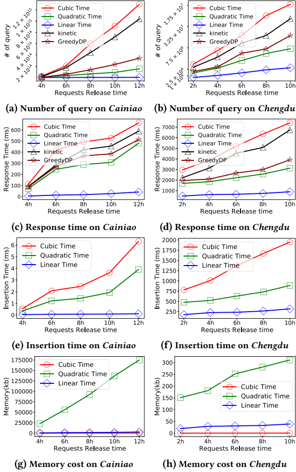
Figure 11: Results of varying requests release time duration
