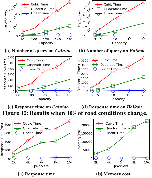
Figure 12: Results when 10% of road conditions change.
