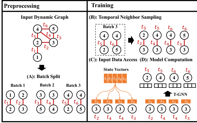
Figure 1: A toy example of T-GNN training. The input dynamic graph contains 6 interactions with different timestamps. The batch size is 2 (2 target interactions), the number of sampled neighbor is 1.
