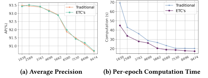
Figure 10: Comparison of (a) average precision and (b) per-epoch computation time between the traditional and ETC’s batching varying the information loss score upper bound on Wiki-Talk dataset.
