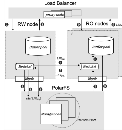
Figure 2: PolarDB Architecture.
