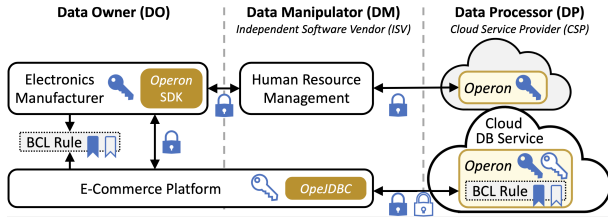
Figure 10: Illustration of supporting the OPDB with Operon . Data owners use their keys (differently colored) to protect data against any application processes or databases. It only performs permitted operations (i.e., by BCL) within TEE.
