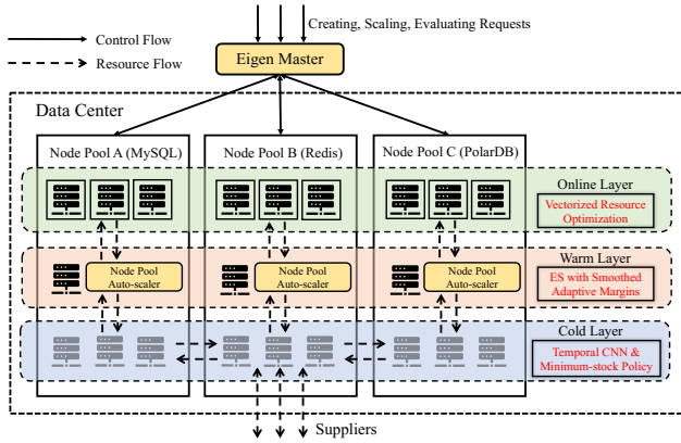
Figure 6: EIGEN’s hierarchical resource management system.
