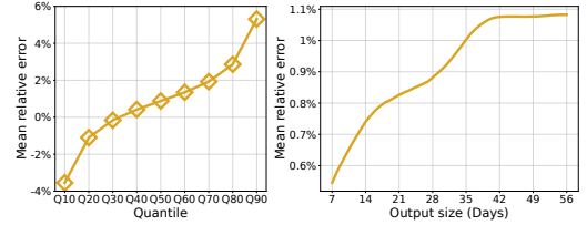
Figure 12: Mean relative error of TCN prediction.
