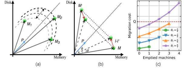
Figure 4: Examples of online allocation (a), instance exchange (b), and binary search of \theta_t (c).
