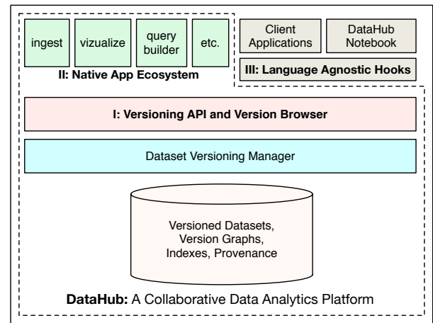
Figure 1: DataHub Architecture
