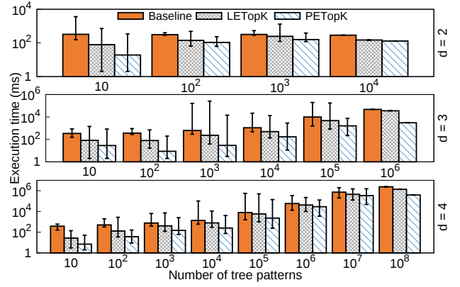
Figure 7: Execution time and number of tree patterns (with height at most d ) for different height threshold d on Wiki
