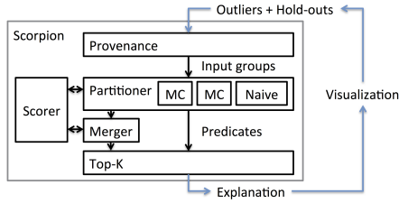
Figure 2: Scorpion architecture
