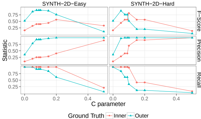
Figure 10: Accuracy statistics of NAIVE as c varies using two sets of ground truth data.
