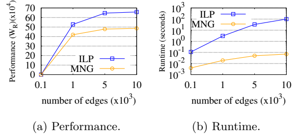
Figure 6: Results on synthetic datasets. (a) Performance as weight of recommendation ( W_R ) of ILP and MNG. (b) Runtime of ILP and MNG (seconds).
