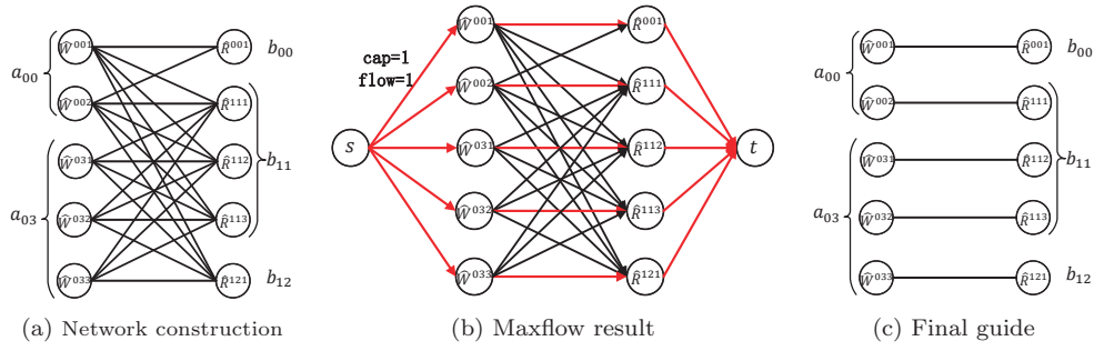
Figure 2: Illustrated example of offline guide generation
