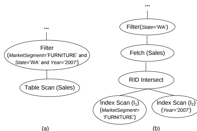
Figure 1. Two alternative plans for a query: (a) Table Scan plan. (b) Index Intersection plan
