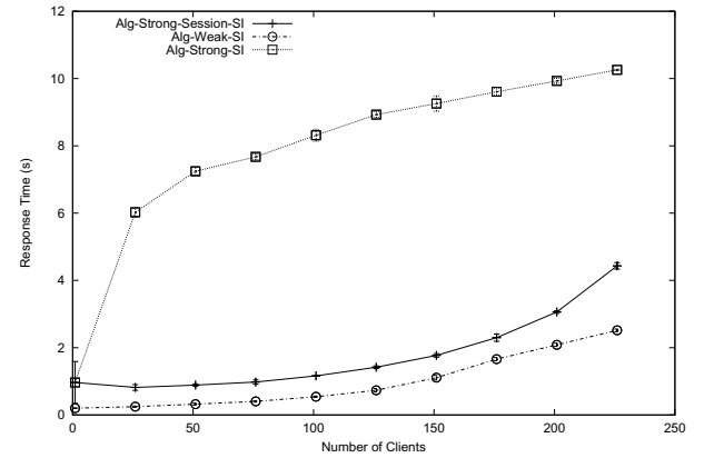
Figure 3: Read-Only Transaction Response Time vs. Number of Clients, 80/20 workload
